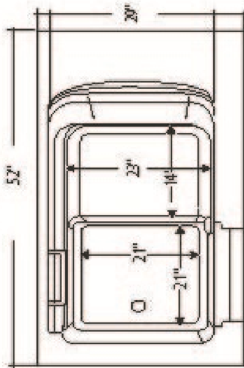
ACCESS PLAN
